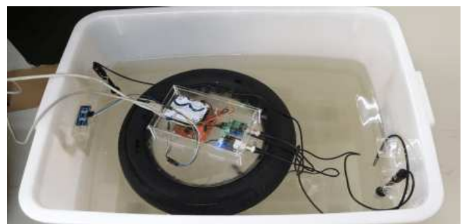
Fig. 6 Initial testing of water sensor for calibration
