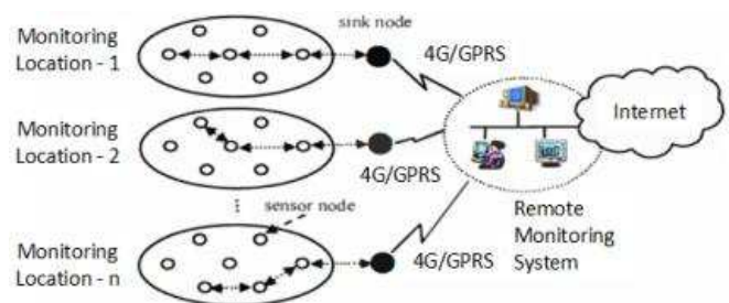
Fig. 5 Communication link of a sensor node to the data gateway system
