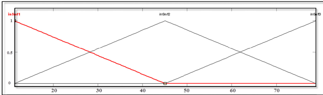
Fig. 3 Membership functions for slope angle
