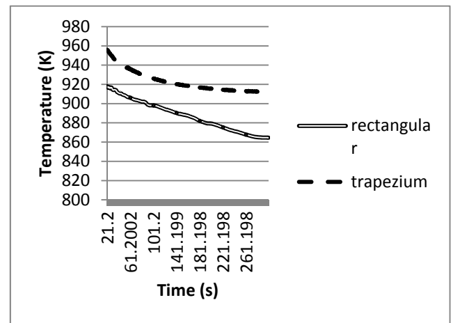
Fig. 5 Cooling curve at point 1
