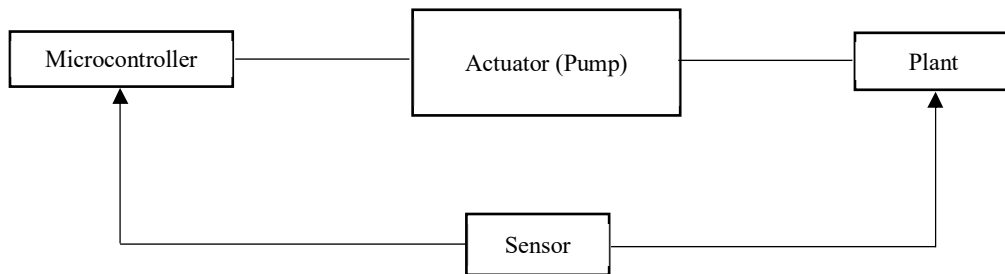
Fig. 3 Software Algorithms
