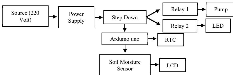
Fig. 4 Block Diagram
