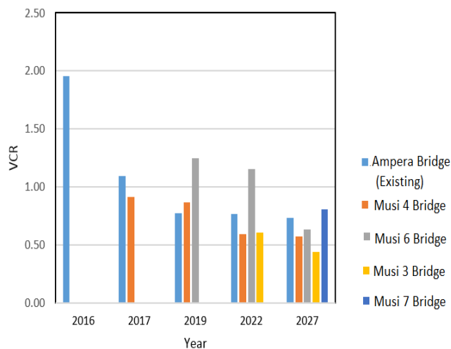
Fig. 8 Service level of bridges
