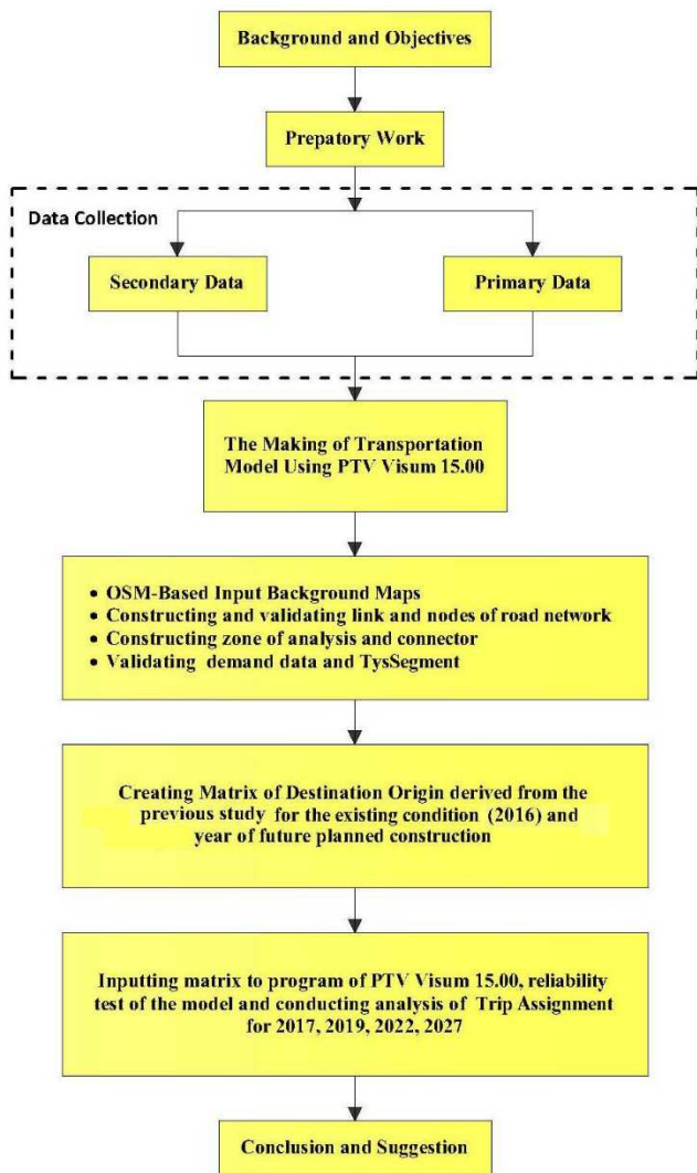
Fig. 2 Research methodology
