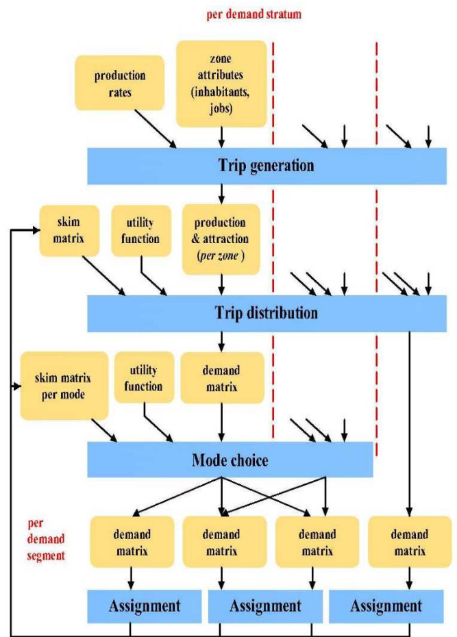
Fig. 1 Integrated 4-step model in visum
