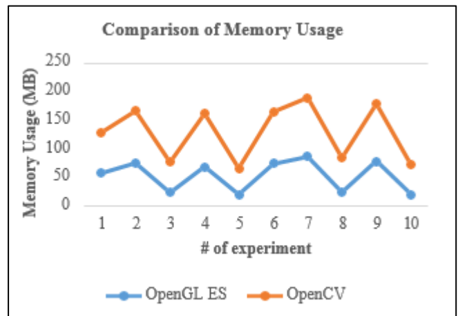
Fig. 8 Comparison of average memory usage between native video filtering using OpenCV and OpenGL ES. OpenGL ES and OpenCV are denoted by the blue and orange line, respectively.
