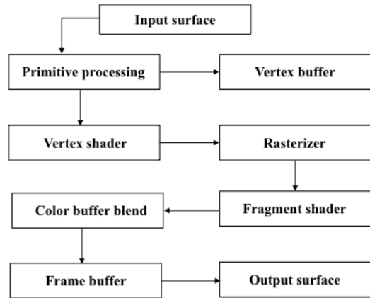
Fig. 4 Flow of frame editing
