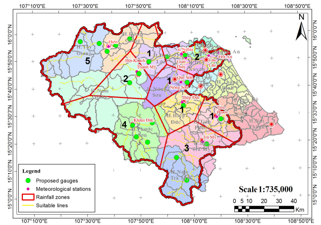
Fig. 2 Meteorological stations network on Vu Gia – Thu Bon river basin
