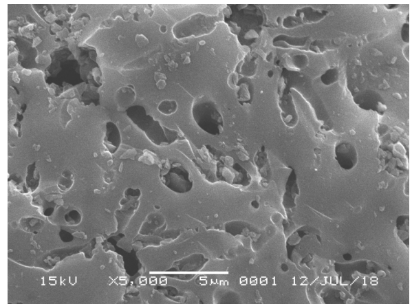
Fig. 10. The scanning electron microscopy (SEM) image of activated carbon of the palm shell with a magnification of 5000x for 1M KOH concentration
