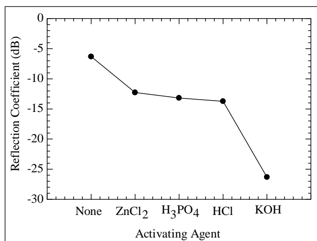
Fig. 4. The maximum reflection coefficient of the activated carbon for several activating agents at a material thickness of 10mm, concentration of 1M and frequency center of 8 GHz.
