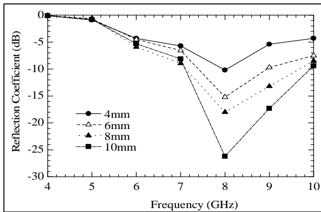
Fig. 7. The relationship between the coefficient of reflection and the frequency using the KOH 1 M activating agent as a variation in thickness from 4 mm to 10 mm.
