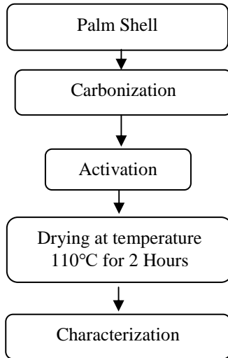
Fig. 1. Step by step of the active carbon production of the palm shell
