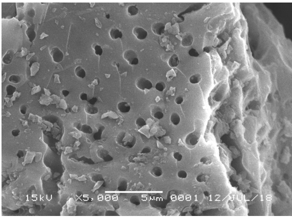
Fig. 11. The scanning electron microscopy (SEM) image of activated carbon of the palm shell with a magnification of 5000x for 5M KOH concentration
