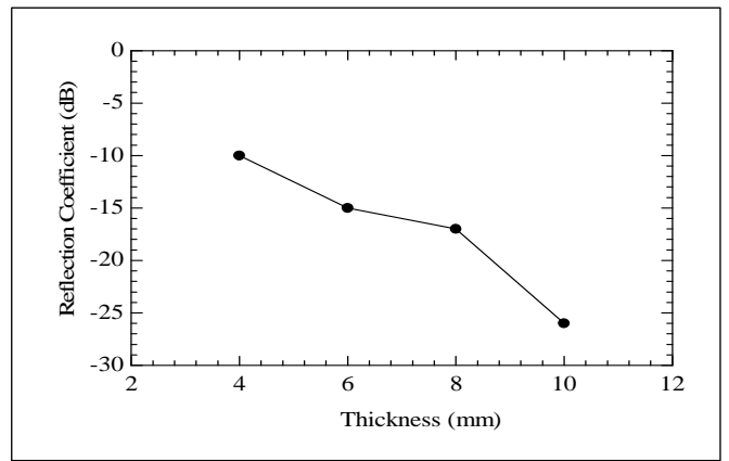
Fig. 8. Dependency between absorption and material thickness of the activated carbon at frequency center of 8 GHz and activating agent of KOH 1M
