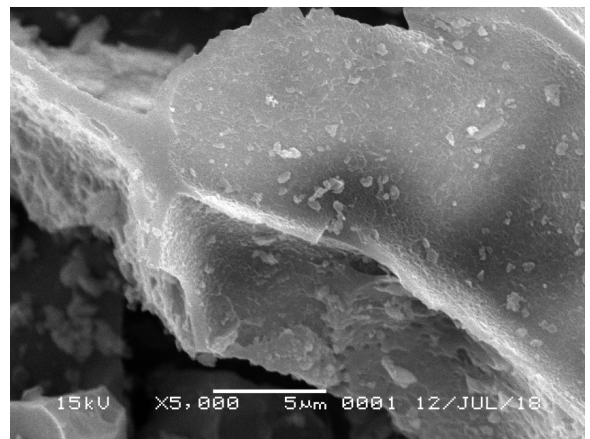
Fig. 9. The scanning electron microscopy (SEM) image of non-activated carbon of the palm shell with a magnification of 5000x
