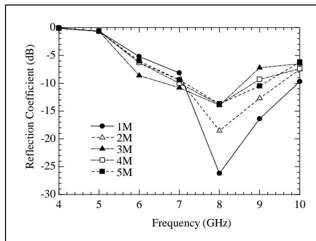
Fig. 5. Measured reflection coefficient of the activated carbon for various concentration of activating agent (1M, 2M, 3M, 4M and 5M) at a material thickness of 10mm.
