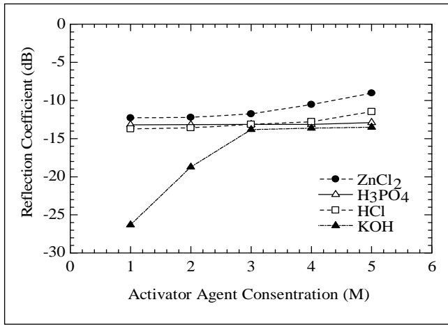
Fig. 6. The relationship between the coefficient of reflection and activating agents concentration at a material thickness of 10mm and frequency center of 8 GHz
