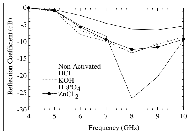
Fig. 3. Measured reflection coefficient of the carbon and the activated carbon with several types of activating agents (HCL, KOH, H 3 PO 4 , and ZnCl 2 ) at a material thickness of 10mm.
